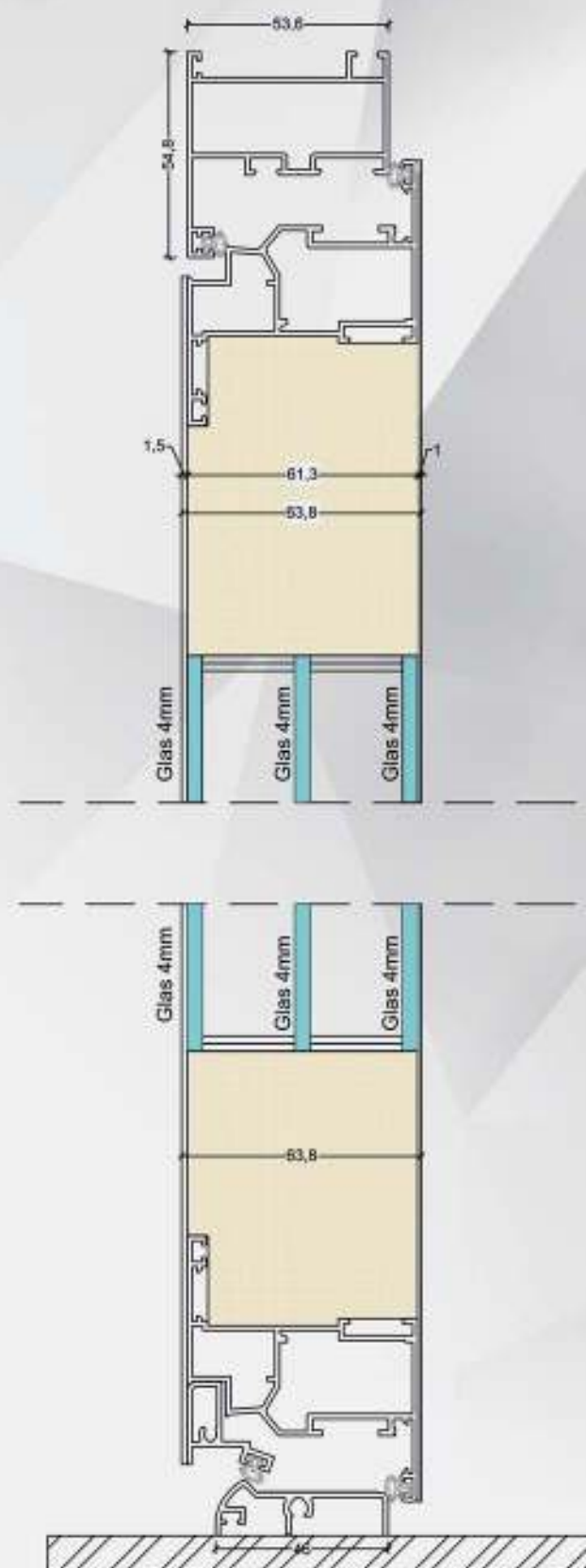
VERTICAL SECTION
